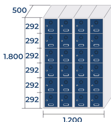
ECOB-30/4 PRO 83kg . 1,08m 3
