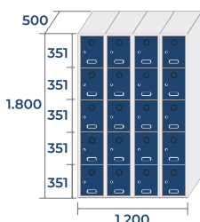
ECOP-30/4 PRO 75,9kg . 1,08m 3
