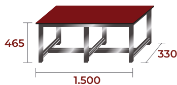
BANC-1-1500-FEN-INOX 18kg · 0,24m 3
